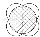
Filo nervato / Ribbed wire Ø (6 ÷ 16 mm)
